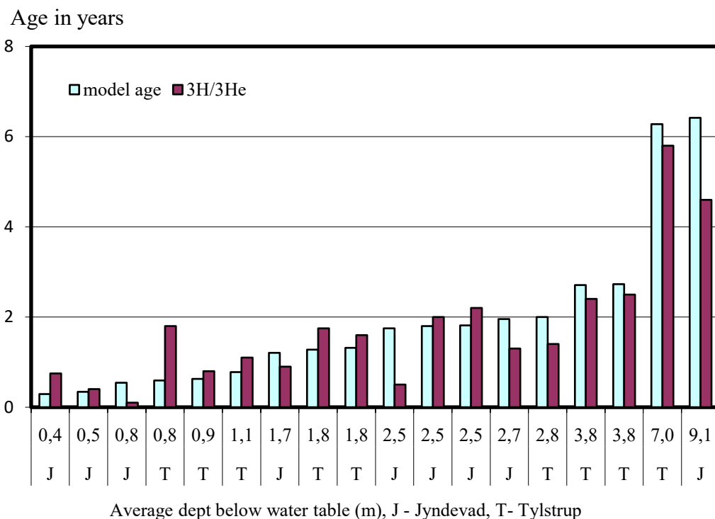
Figure A9.1. Groundwater age at Jydevad and Tylstrup. Recharge model age assumes water velocity of 1.4 m per year, except for the deep filter at Tylstrup (1.1 m per year).
